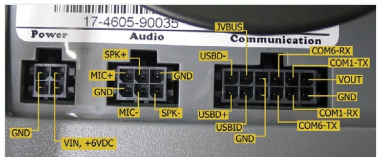
Cradle pinout
